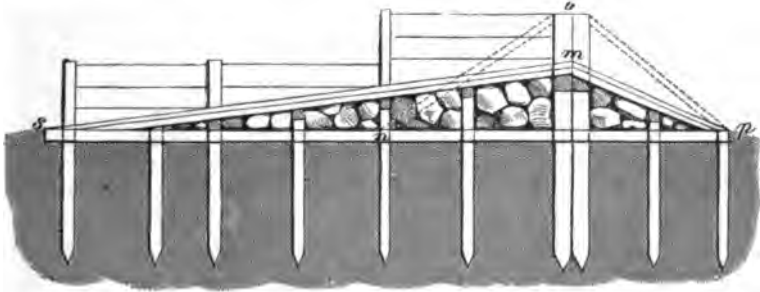
Fig. 247.—Weir with sluice-gates.
